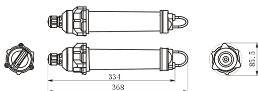
Full plastic explosion-proof equipment light fittings (without steel mesh cover)
