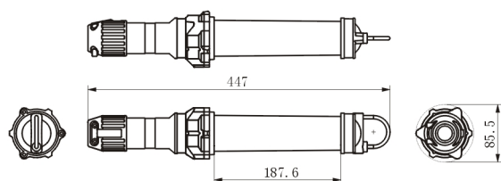
Full plastic explosion-proof overhaul light fittings (without steel mesh cover)
