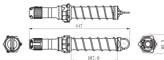
Full plastic explosion-proof overhaul light fittings (with steel mesh cover)
