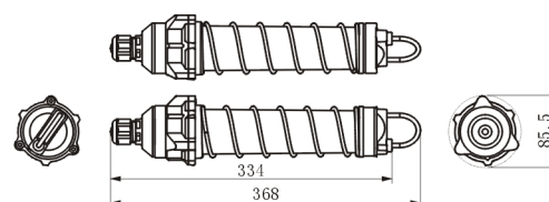
Full plastic explosion-proof equipment light fittings (with steel mesh cover)
